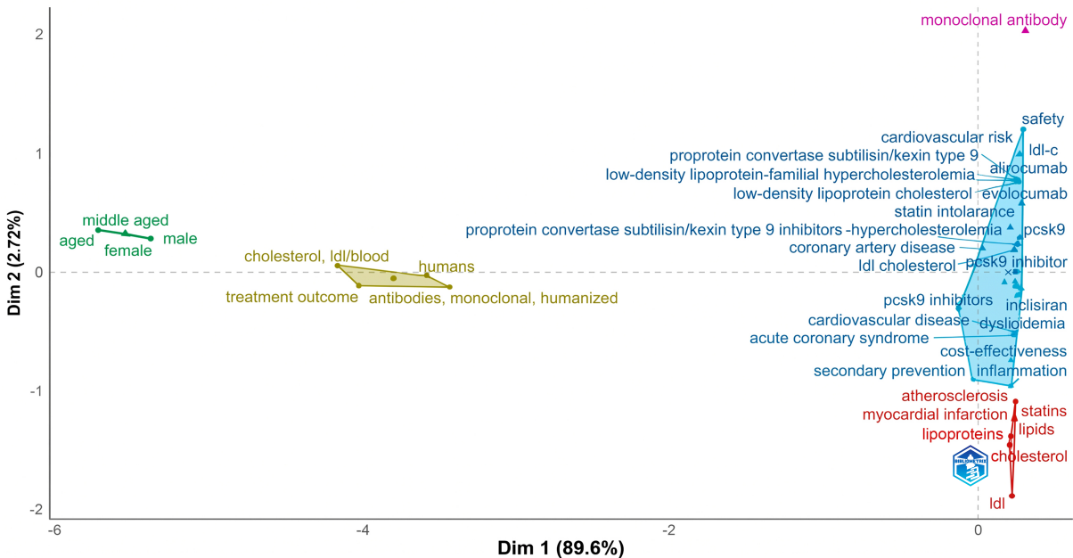
(B) Conceptual Structure Map-method: MCA
