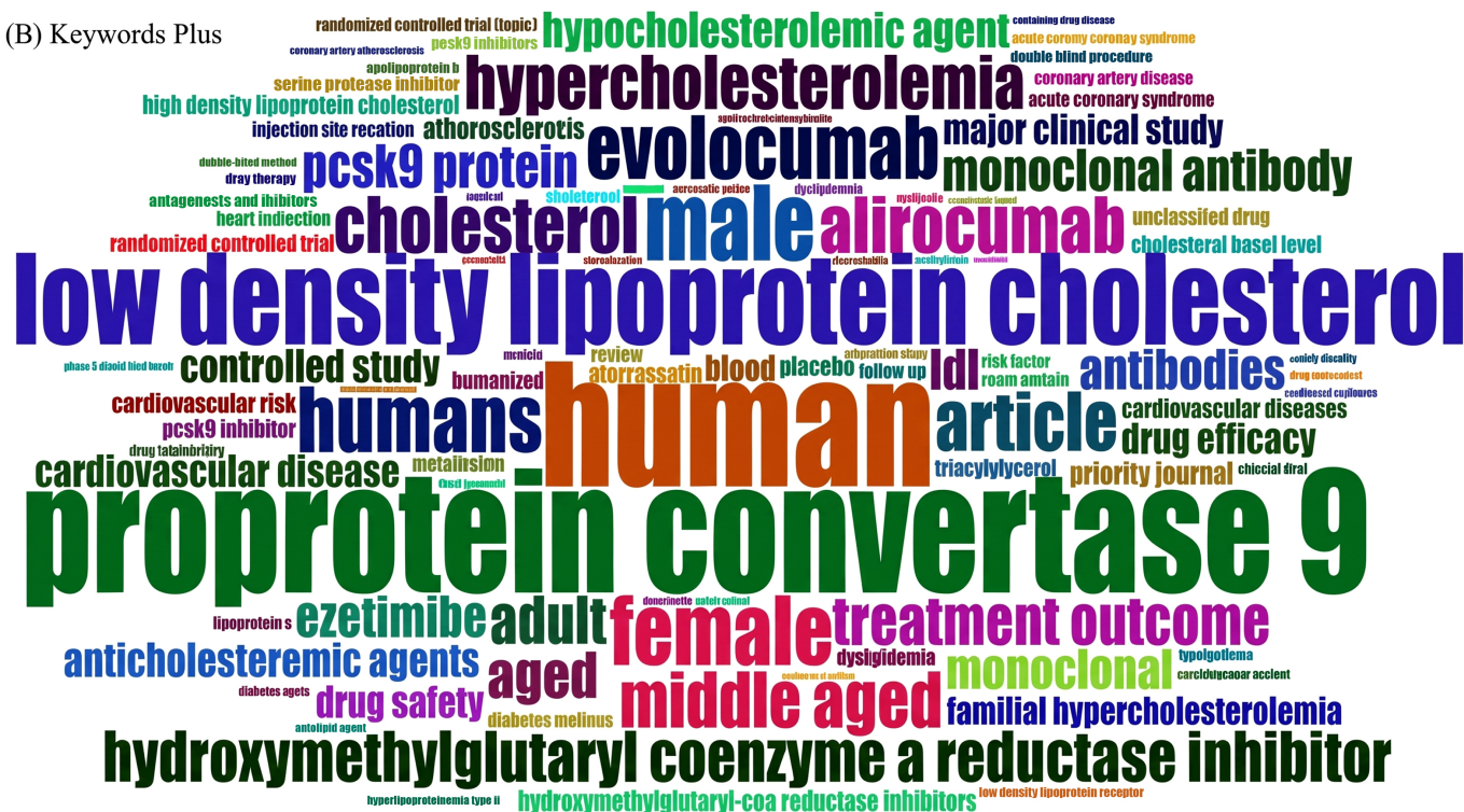
Fig. (4). Word clouds of the top 100 most frequent authors' keywords ( A ) and Keyword Plus terms ( B ) in global PCSK9 inhibitor publications.
