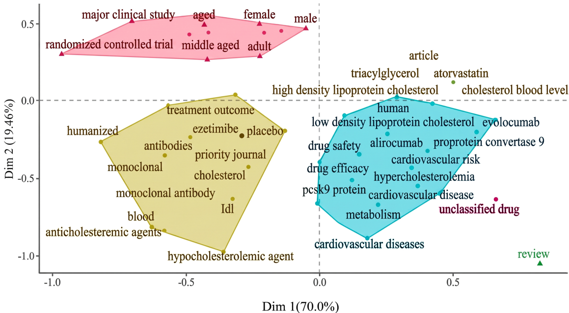
Fig. (6). Factorial analysis using conceptual structure maps generated by multiple correspondence analysis (MCA): authors’ keyword associations (A) and Keywords Plus terms (B).
