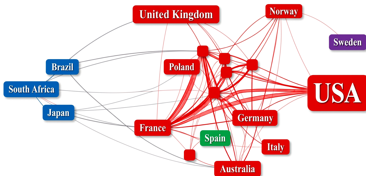
Fig. (3). Collaboration network analysis among the top 50 authors (A), top 50 institutions (B), and top 30 countries (C) contributing to global PCSK9 inhibitor research.
